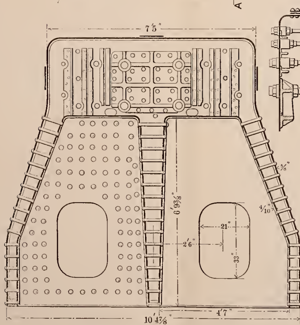
SECTION A-A LOOKING FRONT.
